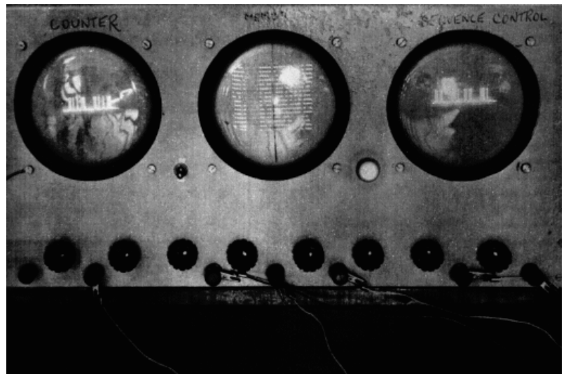
(c) EDSAC monitor tubes showing: left , the Counter; centre , the 32 words in a long tank; right , the Sequence Control Register.
