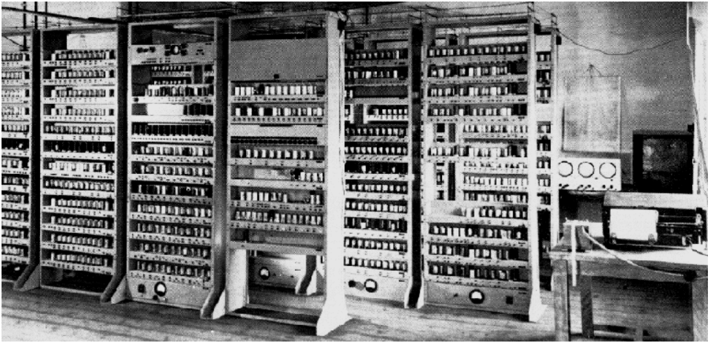
(a) A photograph of the EDSAC taken shortly after its completion in May 1949. The left three-quarters of the picture shows the main racks of the arithmetic unit, control and memory. The input-output equipment (a paper-tape reader and teleprinter) can be seen on the table towards the right. Three of the monitor tubes can be seen to the rear and right of the picture. The EDSAC operated at a speed of approximately 600 operations per second.
